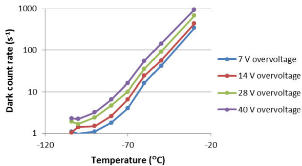
Fig. 1. Dark count rate of Si APD C30902SH vs. temperature, at four different voltages above breakdown voltage.
