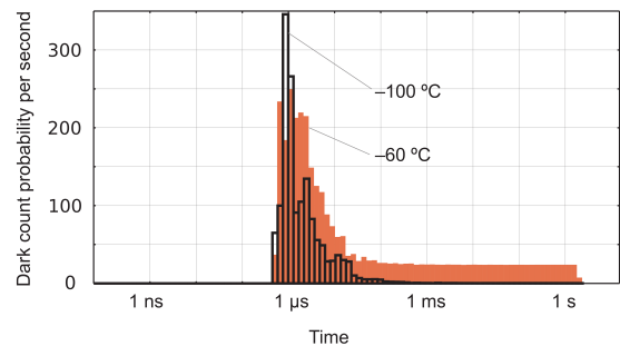
Fig. 2. Dark count probability versus time elapsed since a count, at -60 and -100\text{ }^\circ\text{C} . The first 0.5\text{ }\mu\text{s} is deadtime; the peak is caused by afterpulses; the count probability settles to the dark count rate at long time values.
