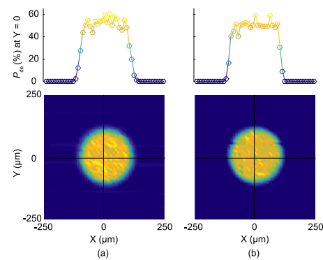
Figure 6 Detection efficiency scan of SLiK-1. (a) Prior to annealing, and (b) after 3.3 W annealing. The spatial profile is essentially unchanged, proving that focused high-power laser illumination does not degrade photosensitivity in the active region of the APD for the power range we tested. The plots at the top are the cross sections at Y = 0 .
